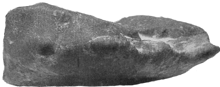
FIG. 12. Flat brustseite (down). Side view showing confirmatory soil line and scoriaceous overflow on back (up). \times 0.76 diameters.
