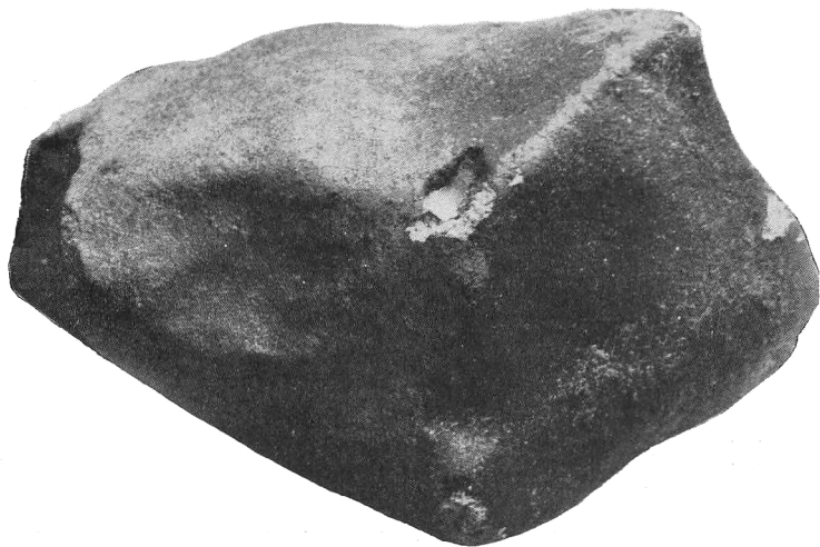
FIG. 10. Piezoglyph formed by burning out of pyrrhotite nodule. × 0.77 diameters.
